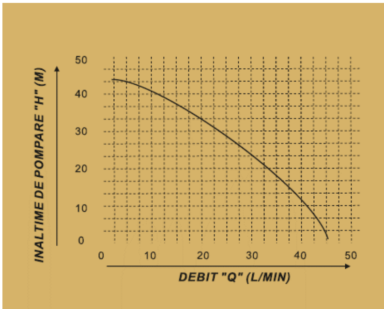
Caracteristica H (m col H 2 O) – Q (l/ min) a pompei JET 150 L
